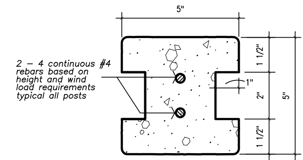
Running Post Section
