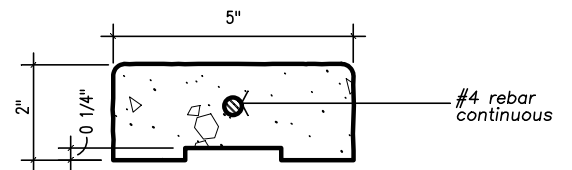
Caprail Section
