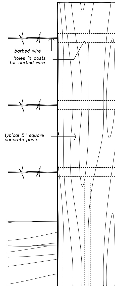
Elevation of Post Top
