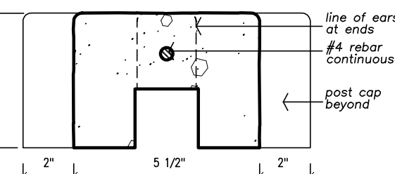
Caprail Section
