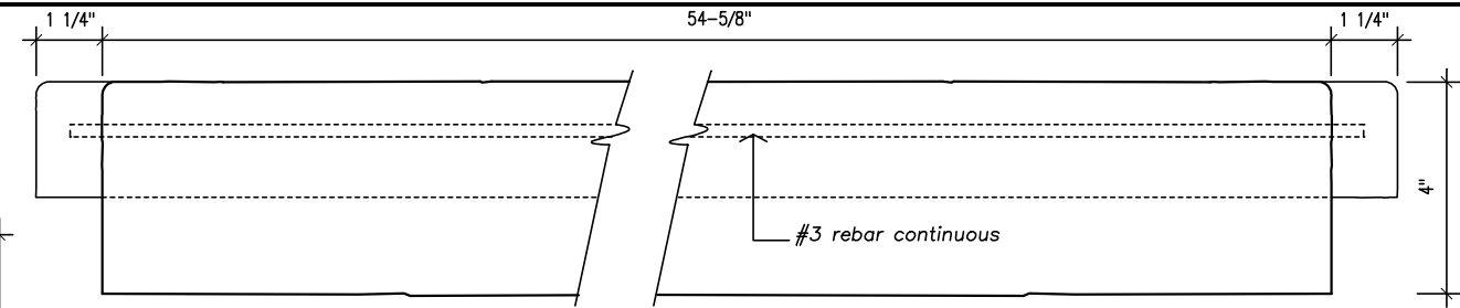
Caprail Elevation
