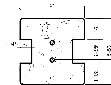
Running Post Section
