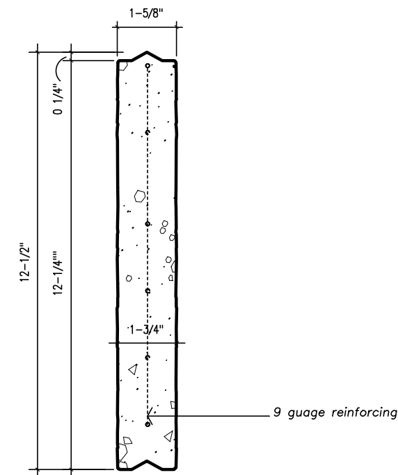
Typical Panel Section
