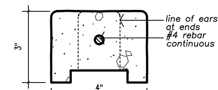
Cap Rail Section
