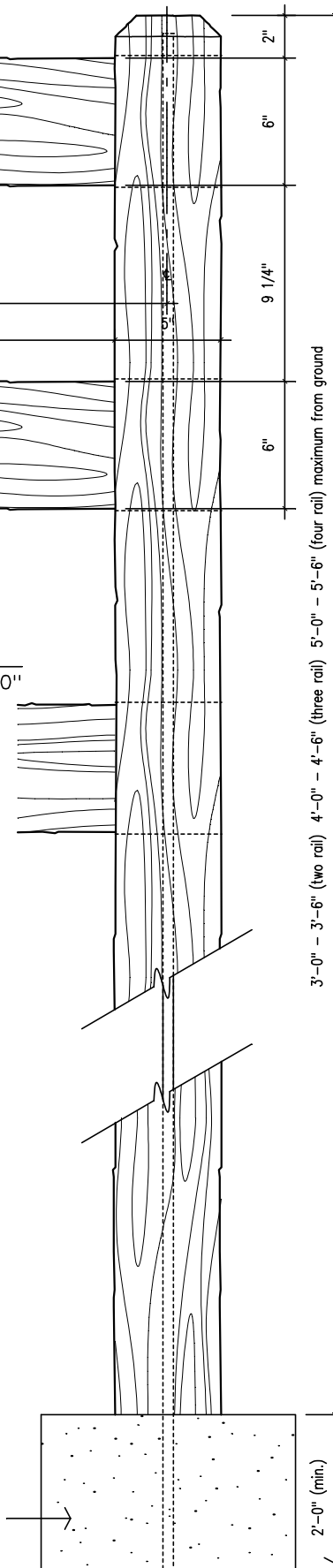
Rail Elevation
