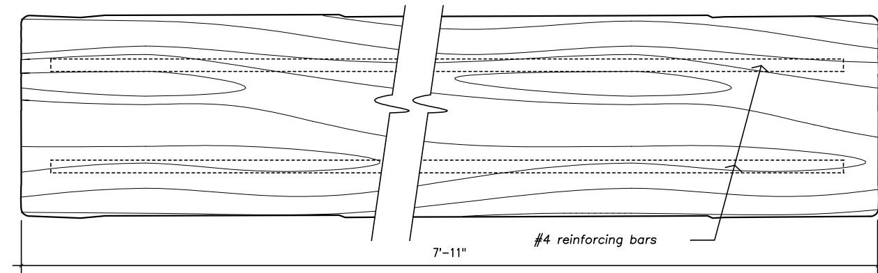
Rail Elevation
