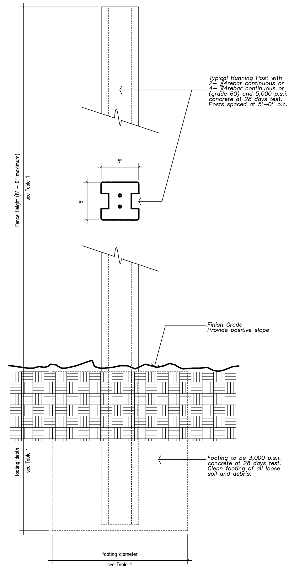
Typical Fence Post Detail
