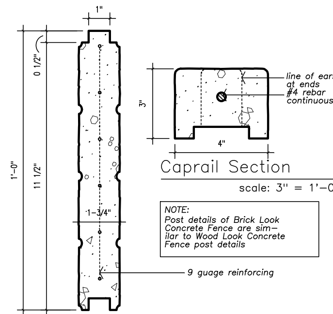
Typical Panel Section
