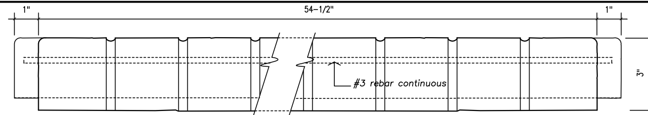
Caprail Elevation
