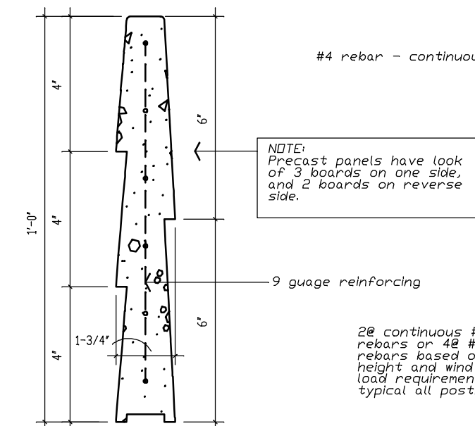
Typical Panel Section
