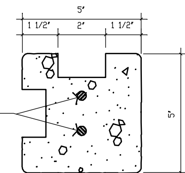
Corner Post Section
