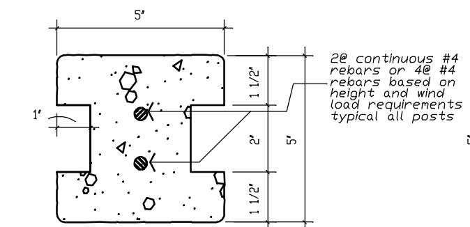
Running Post Section
