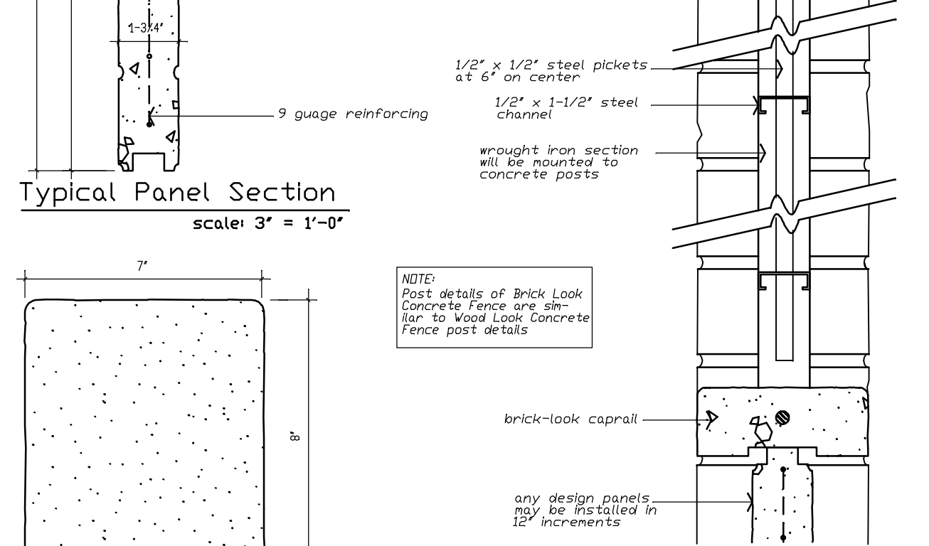
Section Through Fence
